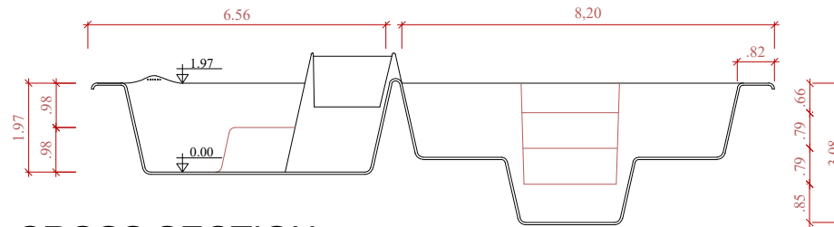
CROSS SECTION SCALE 1:50
