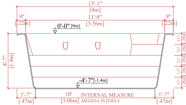
CROSS SECTION CORTE TRANSVERSAL
