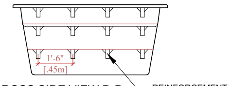
CROSS SIDE VIEW D-D VISTA LATERAL TRANSVERSAL D-D
