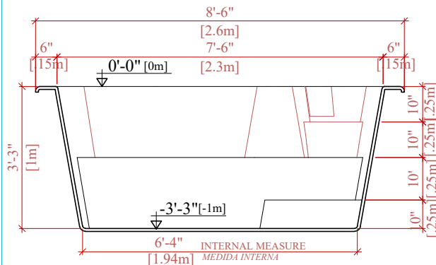
CROSS SECTION CORTE TRANSVERSAL
