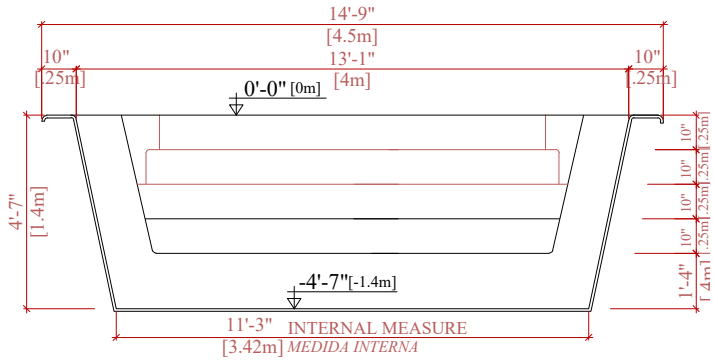
CROSS SECTION CORTE TRANSVERSAL
