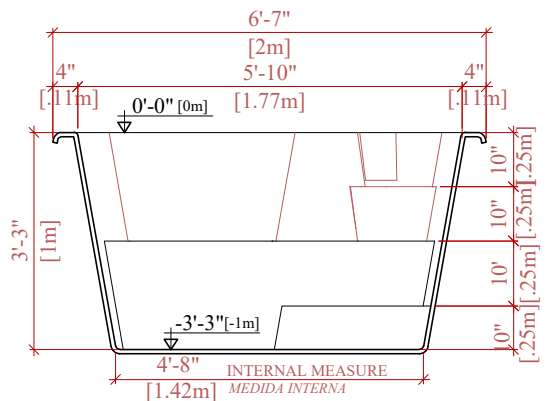
CROSS SECTION CORTE TRANSVERSAL
